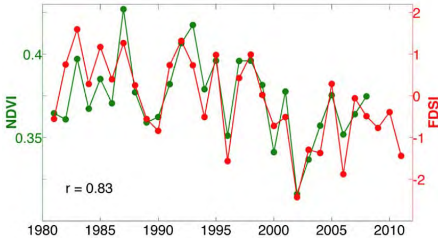
Figure C-8: Correlation between NDVI (summer vegetation greenness index derived from AVHRR satellite imagery) and the Forest Drought-Severity Index (FDSI).
